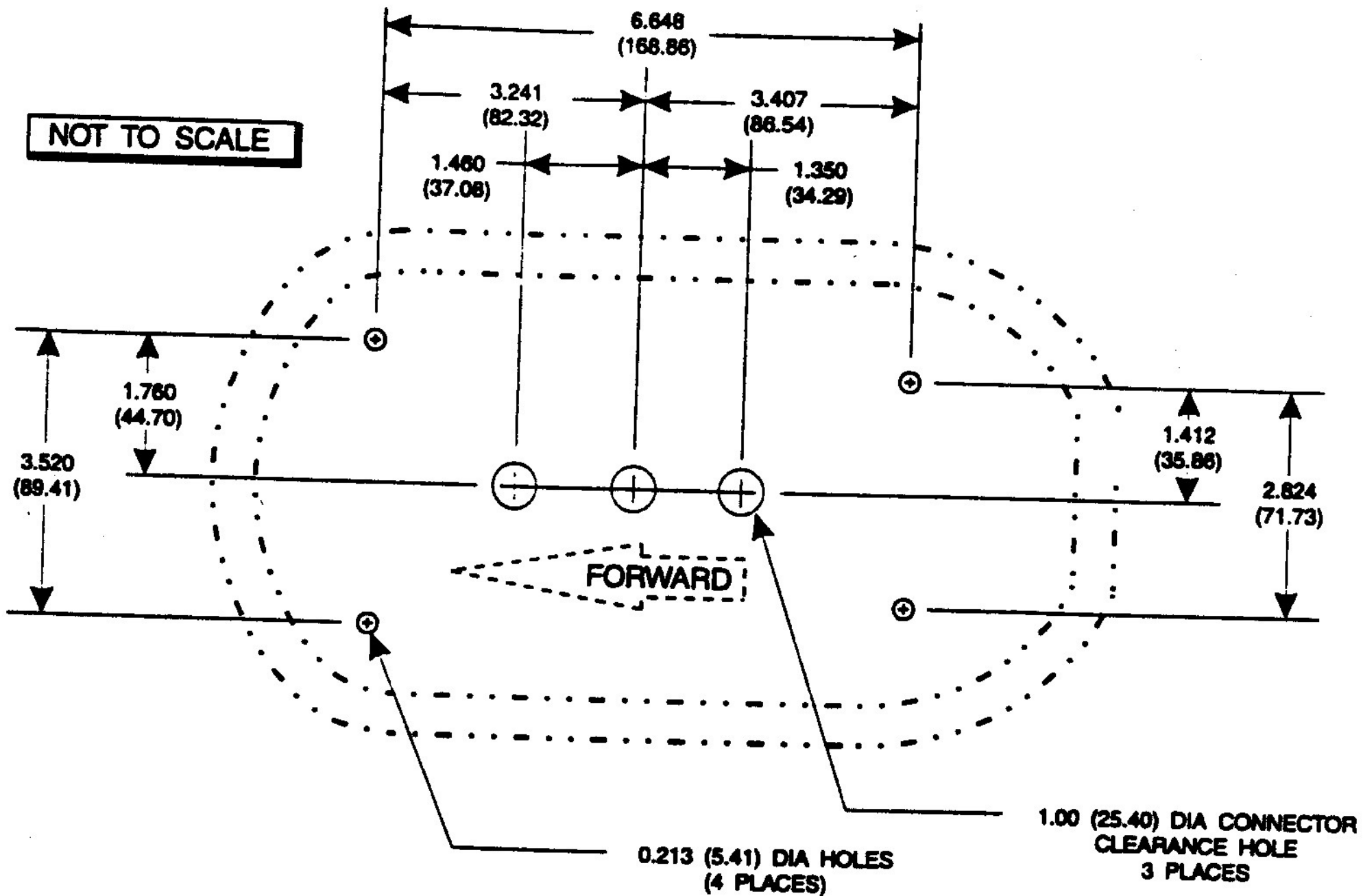
Figure 2-8. Antenna Mounting Holes
